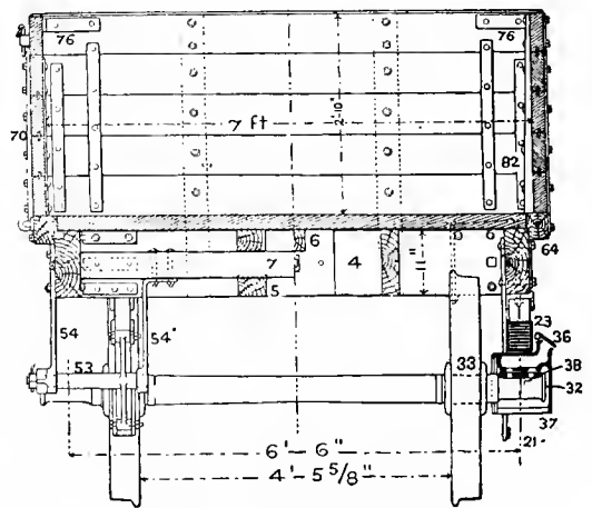
Fig. 351. Transverse Section.
